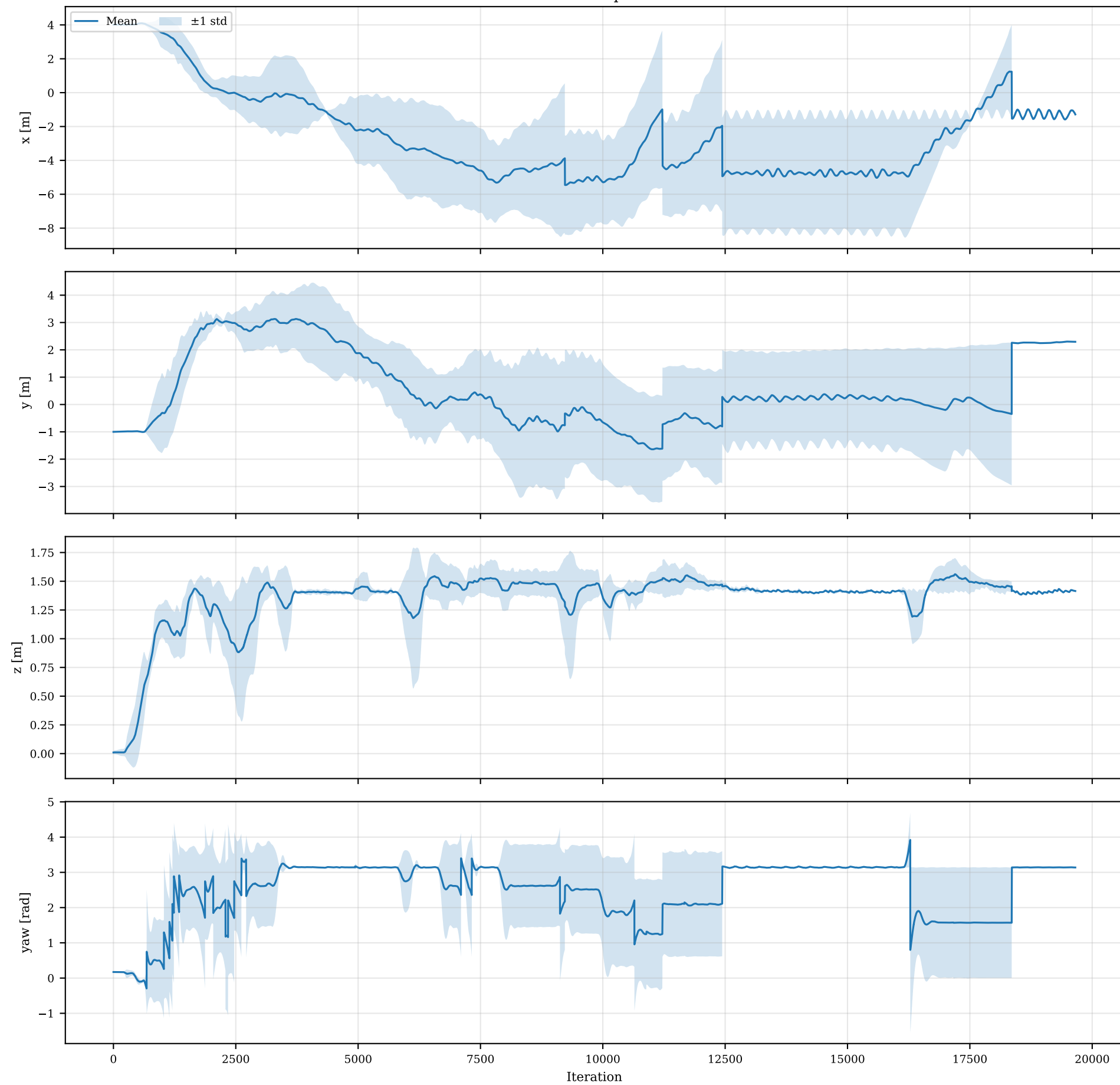
5 UAVS - UAV 31 - Mean position \pm std
